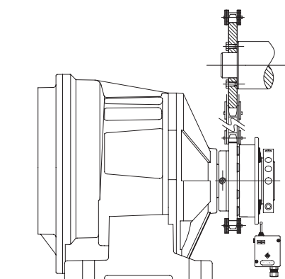
Model EDF/F/C with plate wheel for parallel shaft connections.
