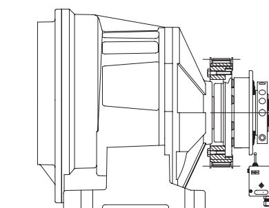
Model EDF/F/F with connection flange integrated to the torque limiter, to fit pulleys, plate wheels, ...
