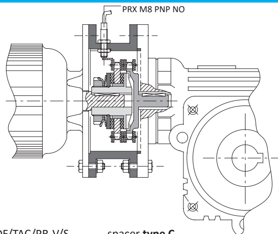
DF/TAC/PR-V/S (with sensor) → spacer type C (with inspection)
